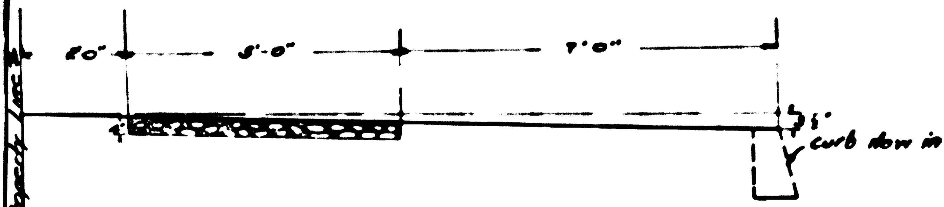
ENLARGED SECTION THROUGH SIDEWALK AT A - A Scale \frac{1}{2}'' = 1'
